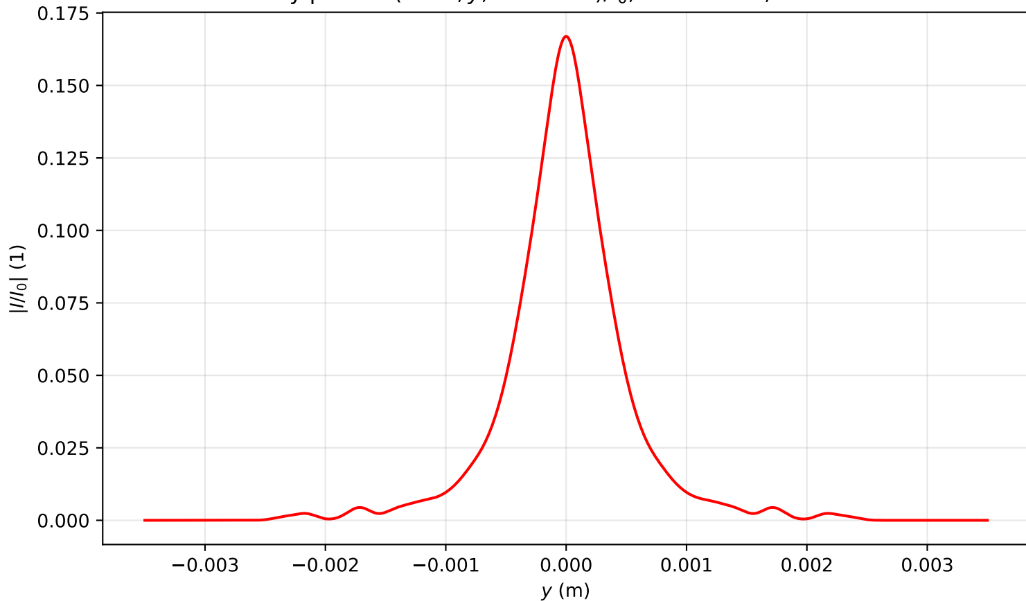
Intensity profile I(x=0, y, z=3.662)/I_0 , \text{Pin}=5.0\text{Pcr} , artificial time
